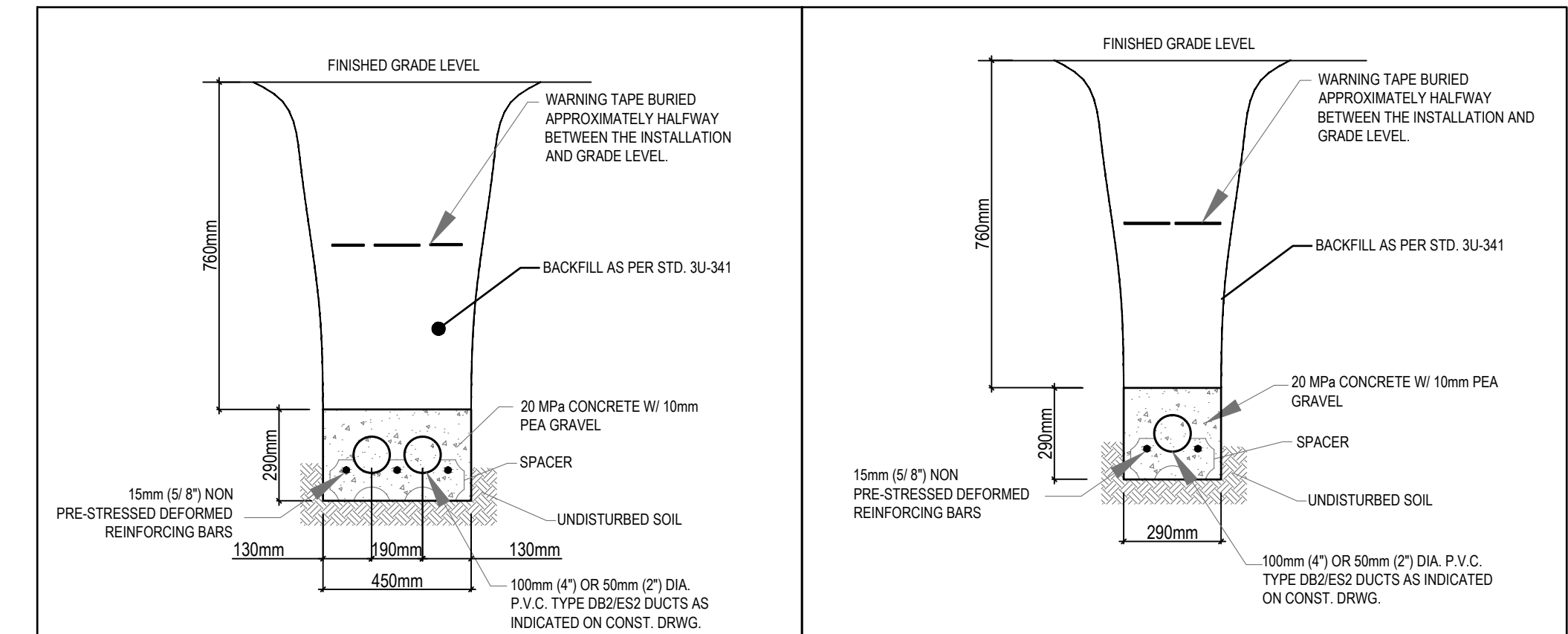
TWO DUCT TYPICAL ARRANGEMENT ENCASED IN CONCRETE DIAGRAM B4-4 DETAIL 2
